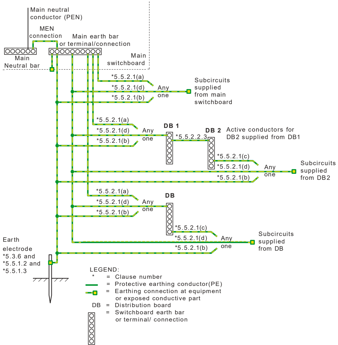
FIGURE 5.3 EXAMPLES OF EARTHING ARRANGEMENTS (CLAUSES 5.5.2.1 AND 5.5.2.3)
