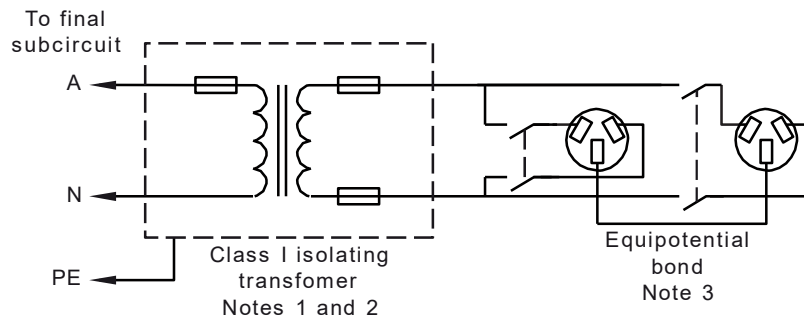
(b) Separated (or isolated) supply with multiple socket-outlets
