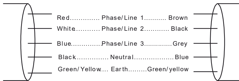
FIGURE 3.2 MULTIPHASE CABLES
