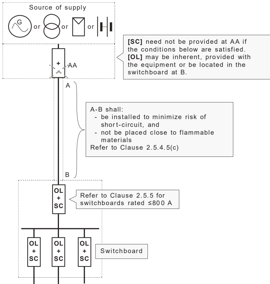
FIGURE 2.9 CONDUCTORS CONNECTING SOURCES OF SUPPLY TO THEIR ASSOCIATED SWITCHBOARD
