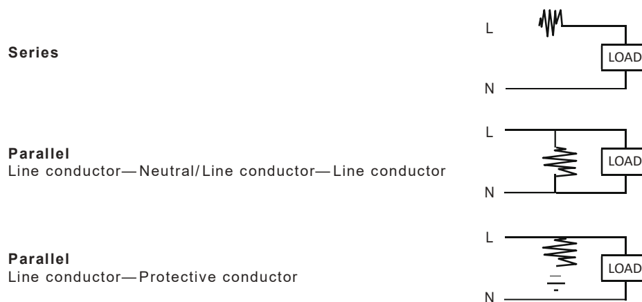
FIGURE O1 TYPES OF ARC FAULT
