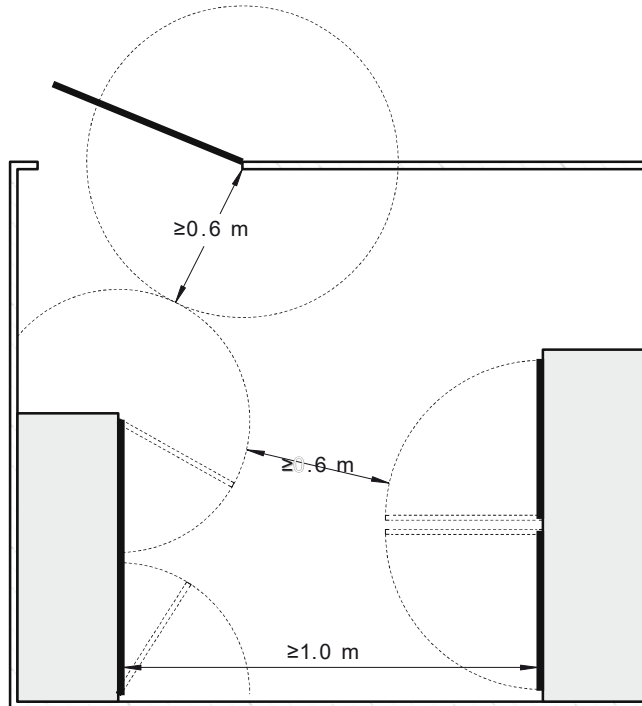
FIGURE 2.23 ACCESS TO SWITCHBOARDS—FACING SWITCHBOARDS
