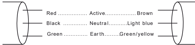
FIGURE 3.1 SINGLE-PHASE CABLES
