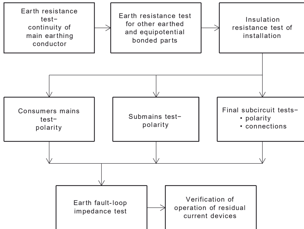
FIGURE 8.1 TESTING SEQUENCE
