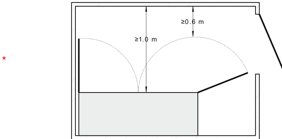
FIGURE 2.20 ACCESS TO SWITCHBOARDS— SWITCHBOARD IN CORNER POSITION
