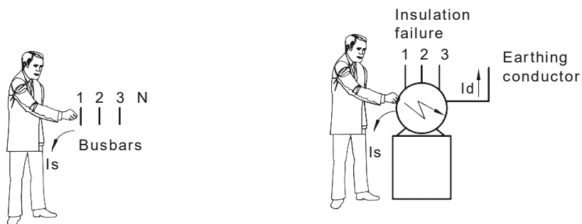
I_s : touch current I_d : fault current (Fault protection required)
